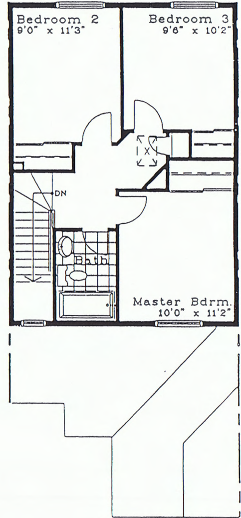
Second Floor
